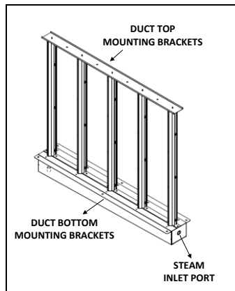
Illustration 7 - Header Mounting Brackets and Steam
