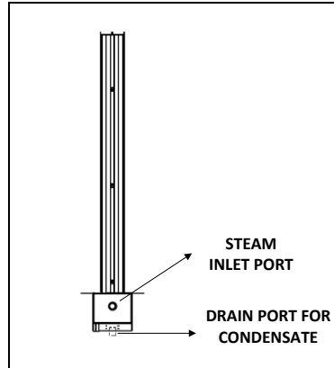
Illustration 5 - Manifold Installation: Front View
